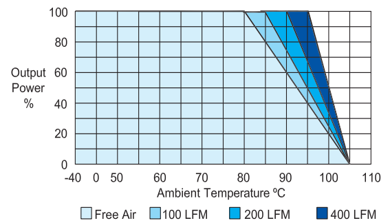
Derating Curve (All other output voltages)
