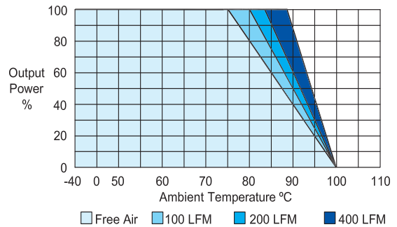
Derating Curve (3.3V, 5V & ±5V)
