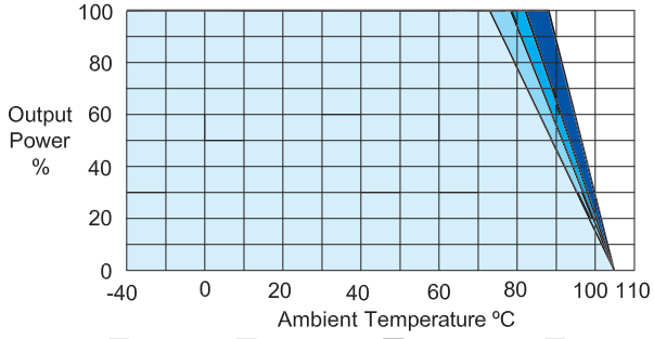
Without Heatsink
