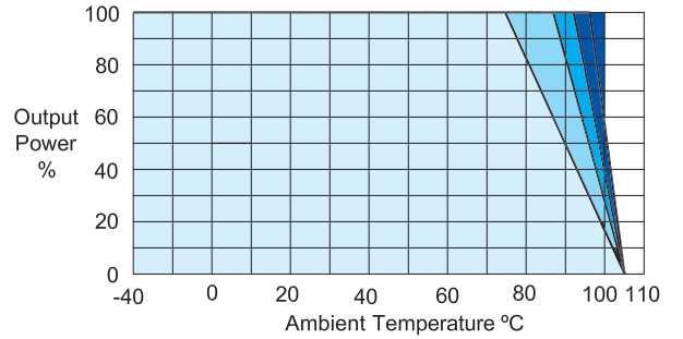
With Heatsink
