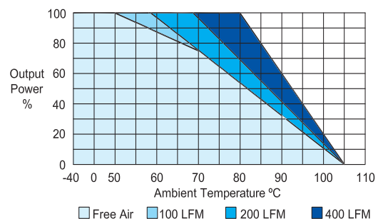
Derating Curve
