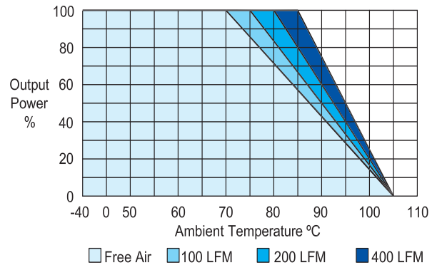
Derating Curve
