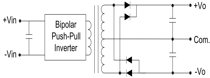
Dual Output Block Diagram
